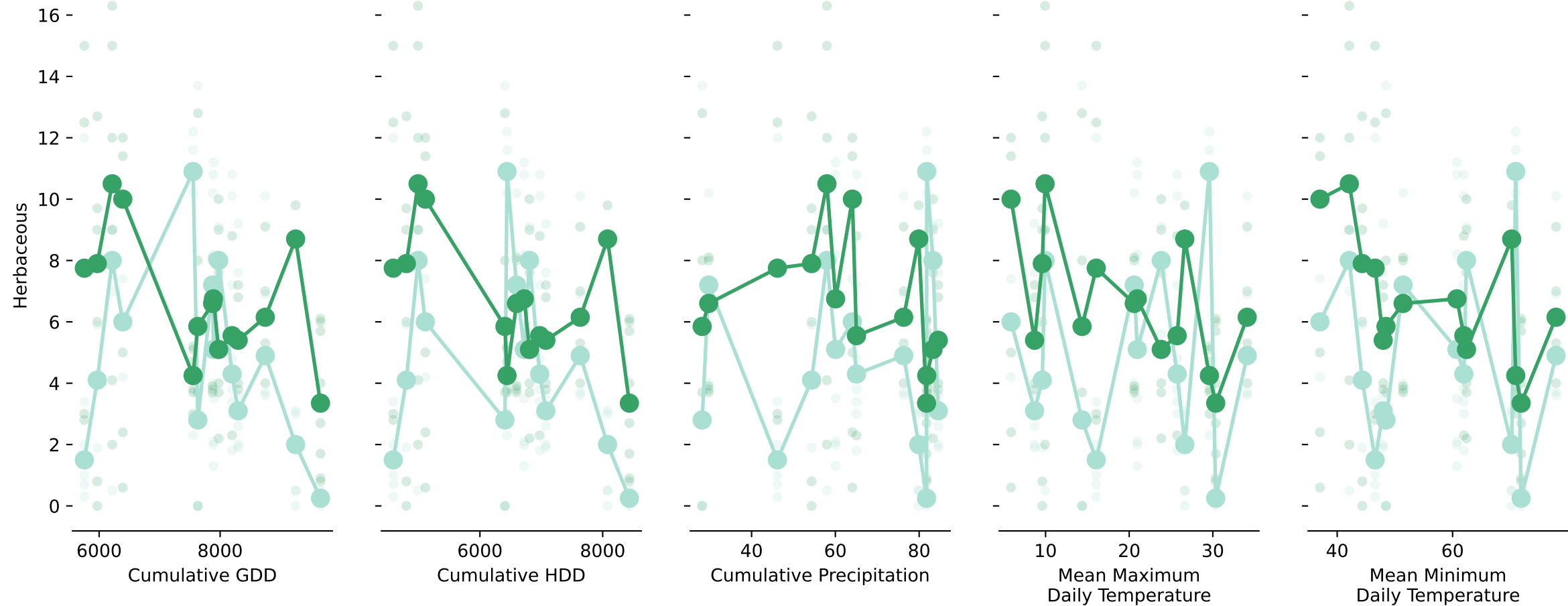
Climate impacts on Herbaceous for Marquette, 2019
